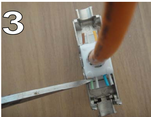
3 Set the modular cover to the module, and cut the wire with scissors to flat
