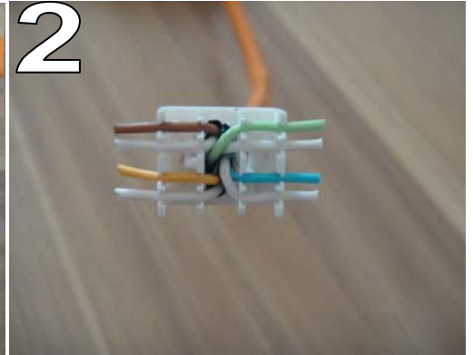
2 Follow the label color on the modular cover, set each wire into proper position, ensure the ground wire connect properly
